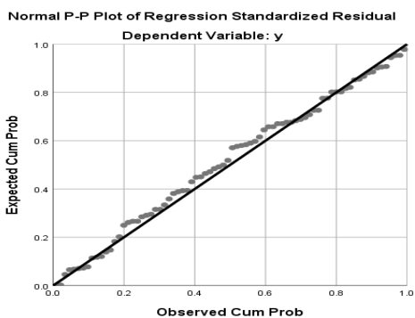
Gambar 2 Scatterplot
